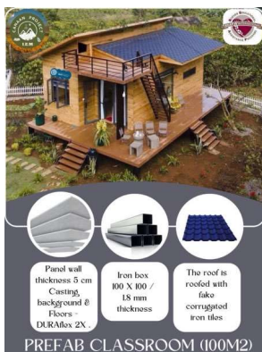
PREFAB CLASSROOM (100M2)
